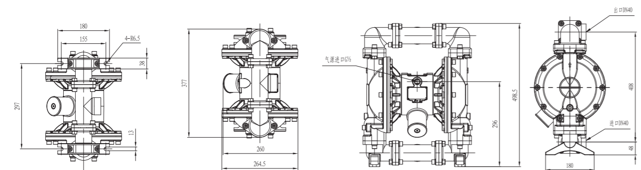
不锈钢/球铁 Stainless steel/Nodular cast iron
