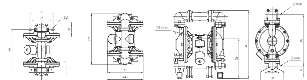
不锈钢/球铁 Stainless steel/Nodular cast iron
