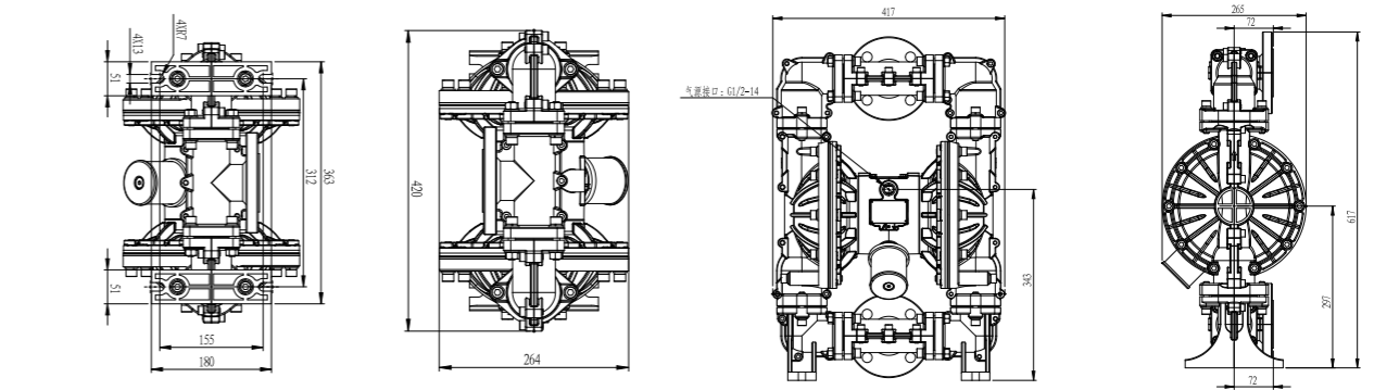
衬氟Lining PVDF
