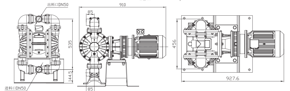
不锈钢/球铁 Stainless steel/Nodular cast iron
