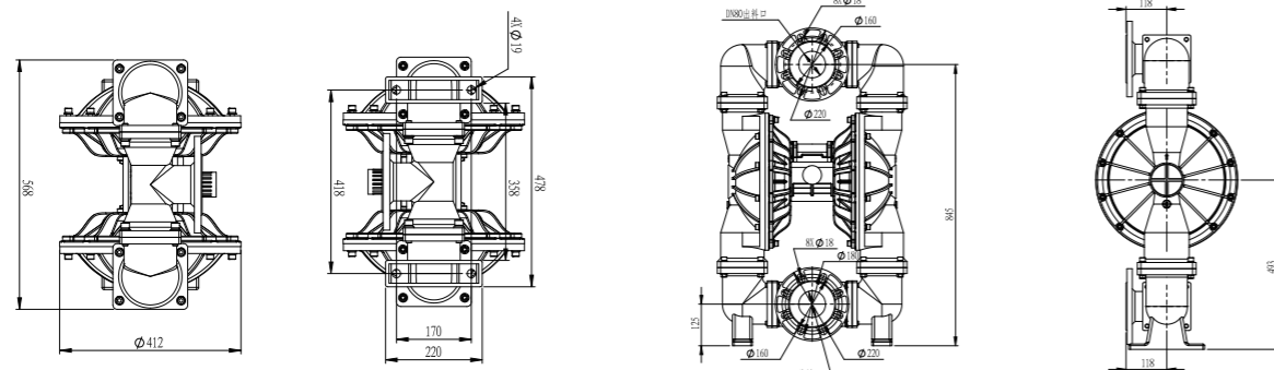
不锈钢/球铁 Stainless steel/Nodular cast iron
