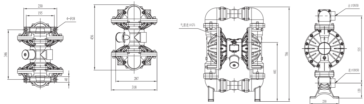
不锈钢 Stainless steel
