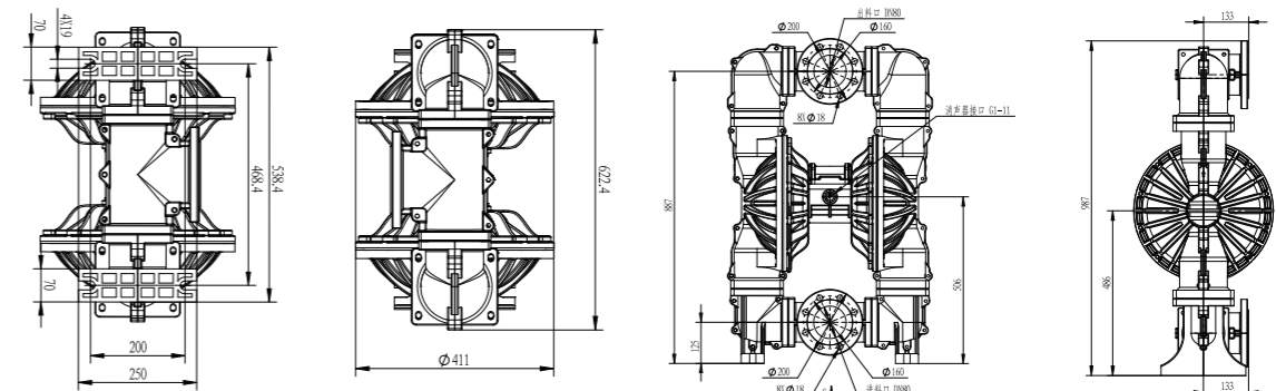
衬氟Lining PVDF
