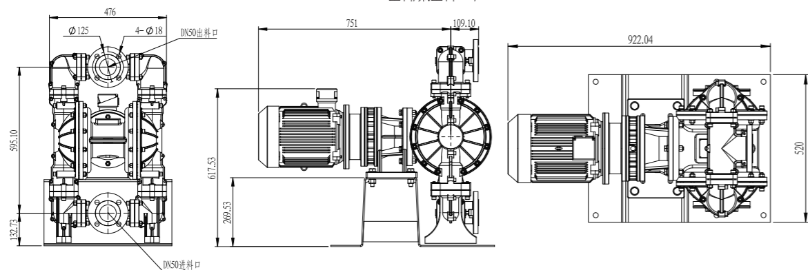
衬氟Lining PVDF
